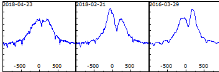
FY CMa
